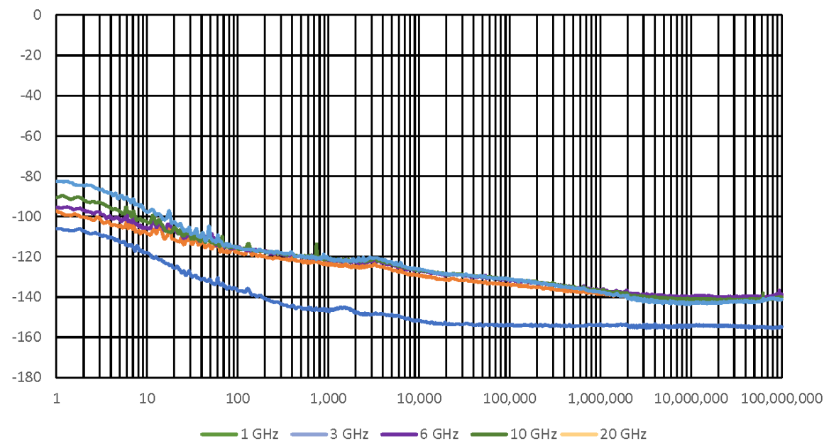
Figure 10. Measured residual phase noise using the external LO mode for N5192A.
