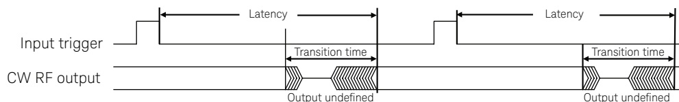
Figure 1. Switching speed definitions with input trigger
