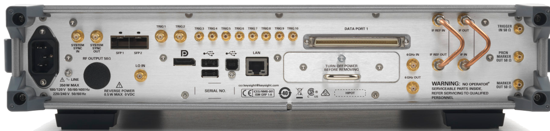
Figure 13. The UXG agile vector adapter rear panel.
