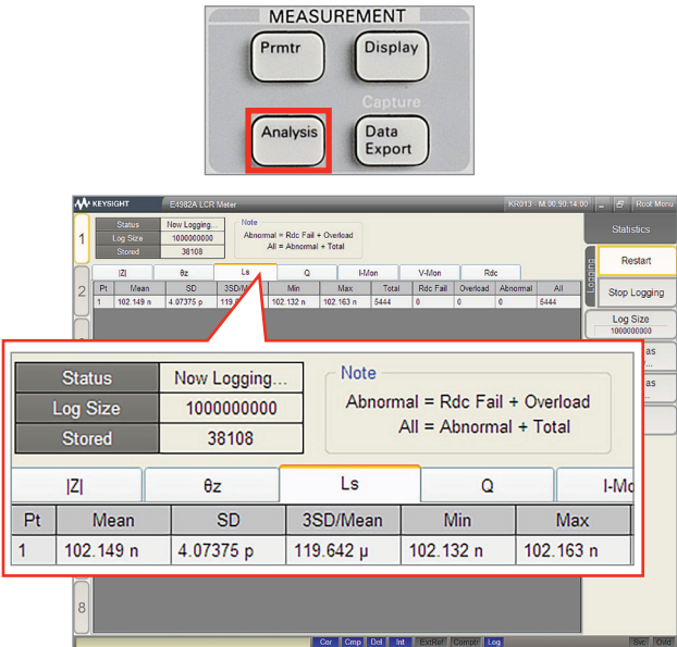
Statistical analysis
