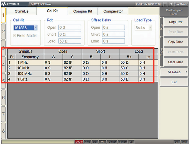
Calibration standard data setup display Different calibration reference values can independently be set at each list measurement frequency
