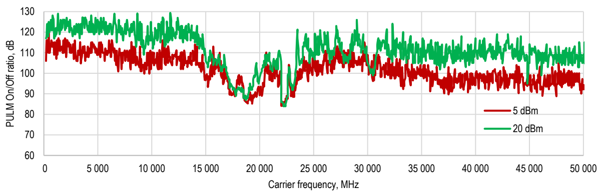
Figure 11. Pulse on/off ratio
