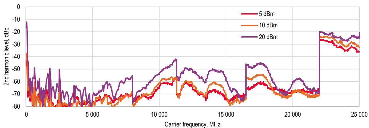
Figure 4. 2 nd Harmonic at different output power
