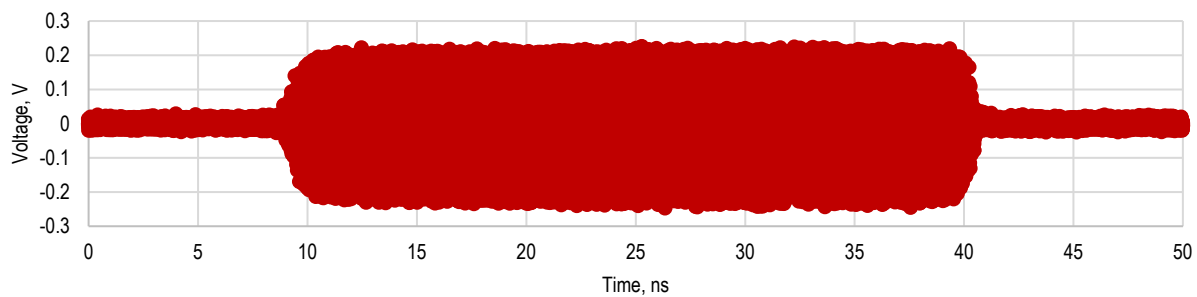
Figure 13. 50 GHz pulse-modulated
