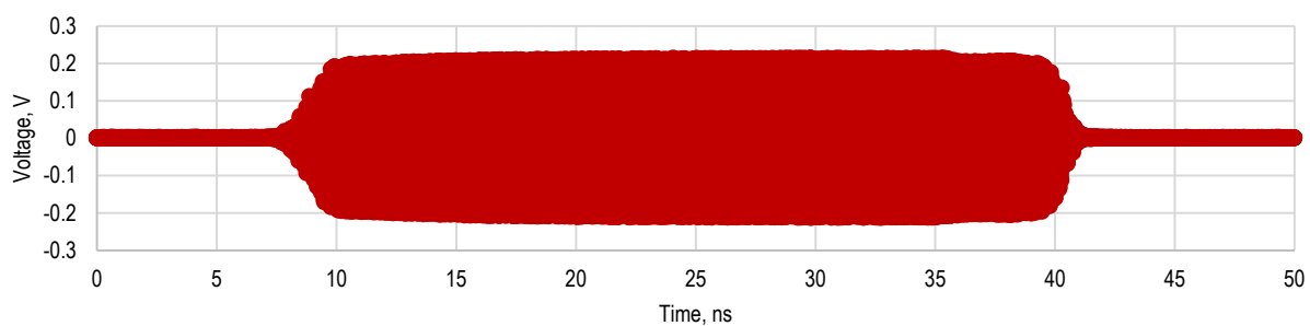
Figure 12. 10 GHz pulse-modulated
