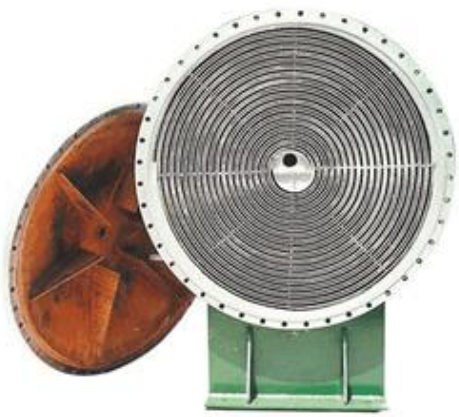
Type II spiral plate heat exchanger
