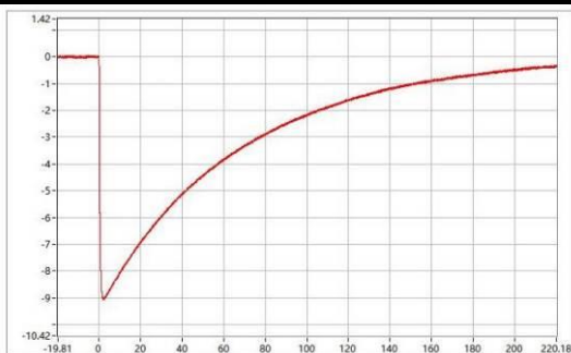
C-06401-25A318-S-WC-009 Upk=-9.04 kV; T1=1.11 us; T2=48.78 us;
