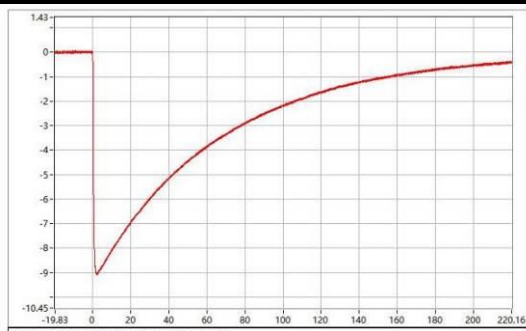
C-06401-25A318-S-WC-050 Upk=-9.06 kV; T1=1.11 us; T2=48.97 us;
