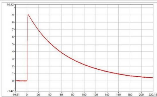
C-06401-25A318-S-WC-013 Upk=9.03 kV; T1=1.11 us; T2=49.59 us;
