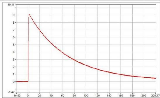
C-06401-25A318-S-WC-014 Upk=9.04 kV; T1=1.11 us; T2=49.92 us;
