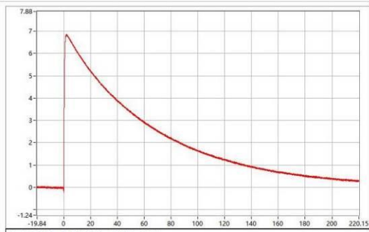
C-06401-25A318-S-WC-052 Upk=6.83 kV; T1=1.11 us; T2=49.27 us;
