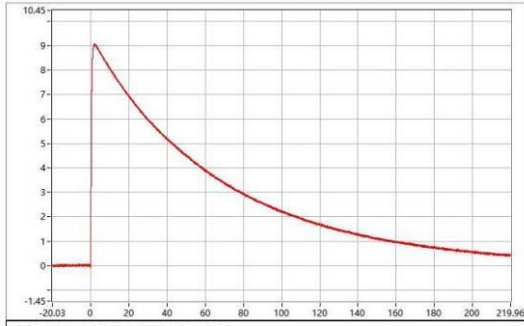
C-06401-25A318-S-WC-023 Upk=9.04 kV; T1=1.10 us; T2=49.87 us;
