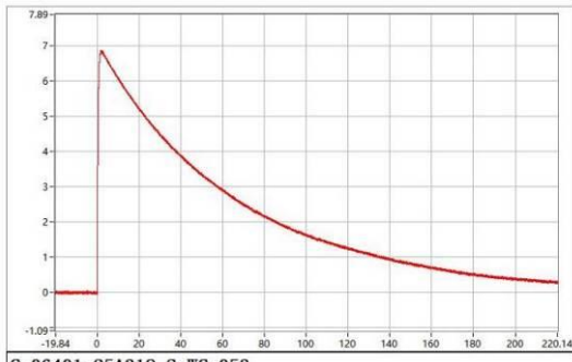
C-06401-25A318-S-WC-053 Upk=6.84 kV; T1=1.11 us; T2=48.74 us;
