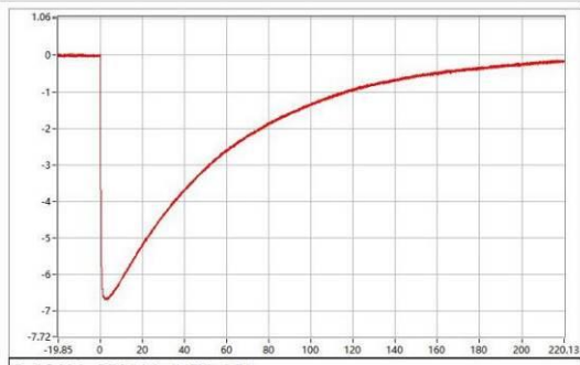
C-06401-25A318-S-WC-070 Upk=-6.68 kV; T1=1.07 us; T2=45.89 us;
