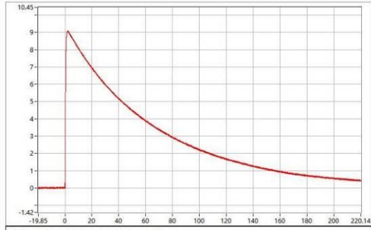
C-06401-25A318-S-WC-024 Upk=9.05 kV; T1=1.10 us; T2=49.26 us;
