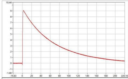
C-06401-25A318-S-WC-032 Upk=9.05 kV; T1=1.10 us; T2=49.06 us;
