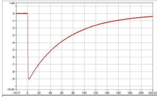
C-06401-25A318-S-WC-030 Upk=-9.05 kV; T1=1.11 us; T2=49.02 us;
