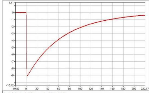
C-06401-25A318-S-WC-028 Upk=-9.03 kV; T1=1.11 us; T2=49.24 us;
