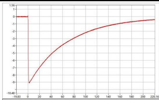
C-06401-25A318-S-WC-026 Upk=-9.05 kV; T1=1.11 us; T2=49.07 us;
