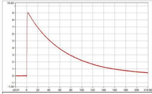
C-06401-25A318-S-WC-022 Upk=9.03 kV; T1=1.10 us; T2=49.66 us;
