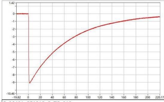
C-06401-25A318-S-WC-019 Upk=-9.06 kV; T1=1.11 us; T2=49.03 us;
