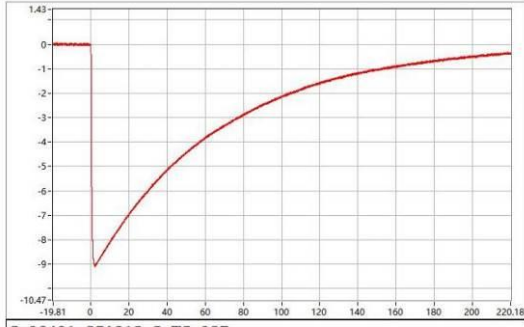
C-06401-25A318-S-WC-027 Upk=-9.04 kV; T1=1.12 us; T2=48.74 us;
