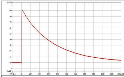
C-06401-25A318-S-WC-031 Upk=9.04 kV; T1=1.10 us; T2=49.43 us;
