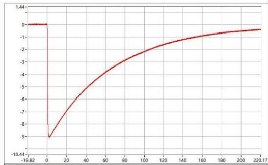
C-06401-25A318-S-WC-016 Upk=-9.05 kV; T1=1.11 us; T2=48.84 us;
