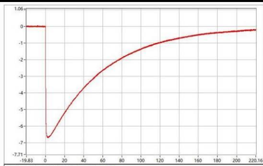
C-06401-25A318-S-WC-066 Upk=-6.68 kV; T1=1.06 us; T2=46.48 us;
