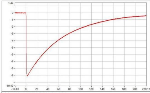
C-06401-25A318-S-WC-029 Upk=-9.07 kV; T1=1.11 us; T2=49.18 us;
