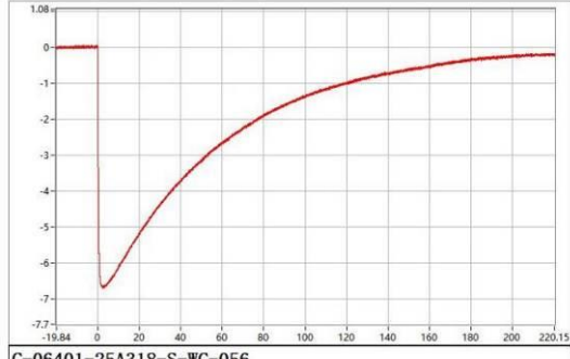
C-06401-25A318-S-WC-056 Upk=-6.66 kV; T1=1.06 us; T2=46.72 us;
