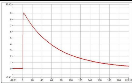
C-06401-25A318-S-WC-025 Upk=9.03 kV; T1=1.11 us; T2=49.62 us;
