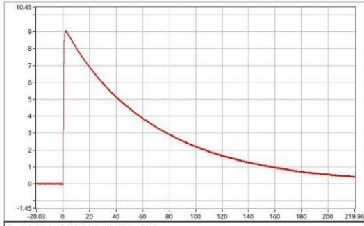
C-06401-25A318-S-WC-021 Upk=9.04 kV; T1=1.10 us; T2=49.46 us;
