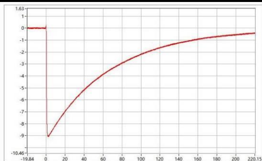
C-06401-25A318-S-WC-010 Upk=-9.05 kV; T1=1.10 us; T2=49.08 us;
