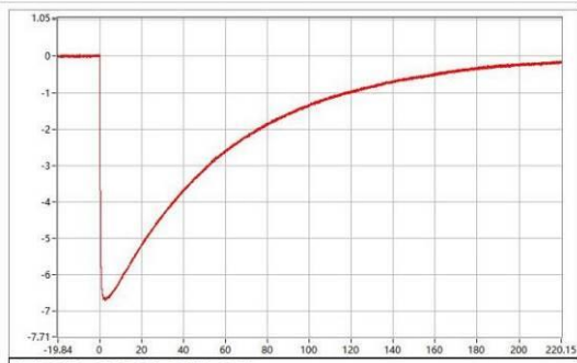
C-06401-25A318-S-WC-068 Upk=-6.68 kV; T1=1.07 us; T2=46.06 us;
