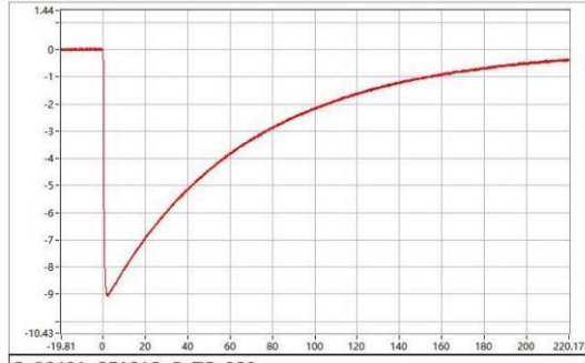
C-06401-25A318-S-WC-020 Upk=-9.04 kV; T1=1.11 us; T2=48.84 us;
