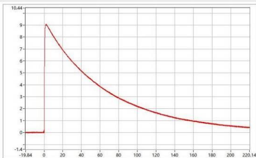
C-06401-25A318-S-WC-011 Upk=9.04 kV; T1=1.10 us; T2=49.06 us;
