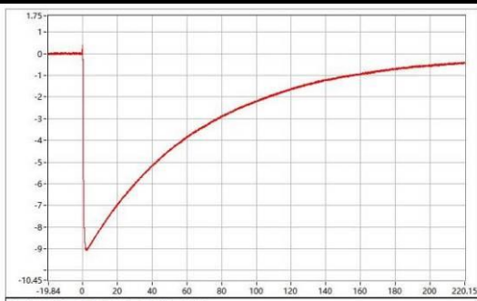
C-06401-25A318-S-WC-017 Upk=-9.06 kV; T1=1.11 us; T2=49.02 us;
