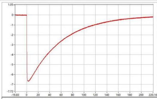
C-06401-25A318-S-WC-069 Upk=-6.67 kV; T1=1.07 us; T2=46.45 us;
