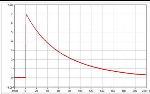
C-06401-25A318-S-WC-065 Upk=6.89 kV; T1=1.10 us; T2=47.22 us;
