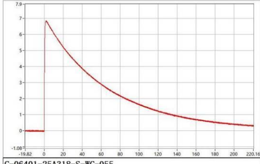
C-06401-25A318-S-WC-055 Upk=6.84 kV; T1=1.11 us; T2=48.91 us;
