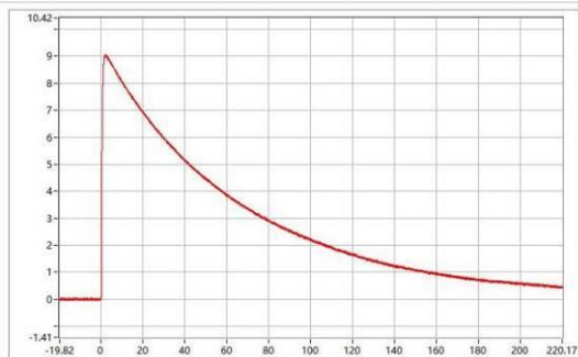
C-06401-25A318-S-WC-012 Upk=9.03 kV; T1=1.10 us; T2=49.08 us;
