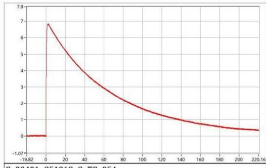
C-06401-25A318-S-WC-054 Upk=6.82 kV; T1=1.11 us; T2=48.85 us;
