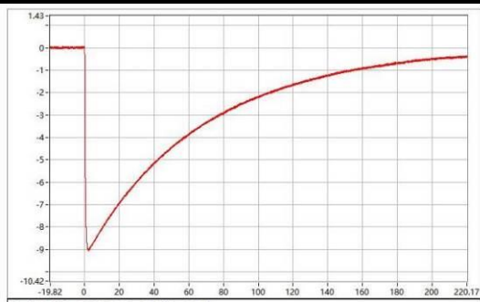
C-06401-25A318-S-WC-018 Upk=-9.03 kV; T1=1.11 us; T2=49.39 us;
