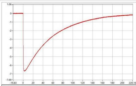
C-06401-25A318-S-WC-067 Upk=-6.67 kV; T1=1.07 us; T2=46.24 us;
