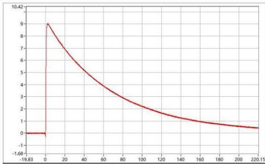
C-06401-25A318-S-WC-015 Upk=9.03 kV; T1=1.10 us; T2=49.71 us;
