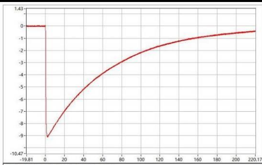
C-06401-25A318-S-WC-049 Upk=-9.06 kV; T1=1.11 us; T2=49.36 us;
