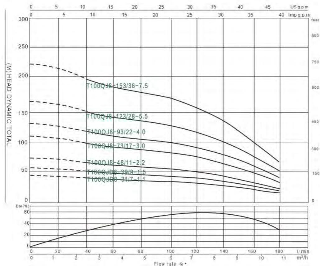
T100/ST100 QJ(D)8 PERFORMANCE DATA 50Hz
