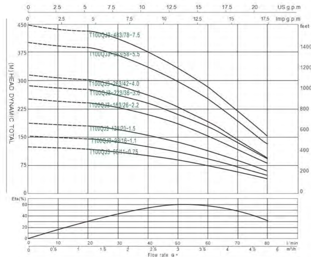
T100/ST100 QJ(D)3 PERFORMANCE DATA 50Hz
