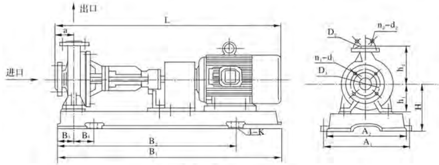
机组安装尺寸图 Diagram of Machine Groups Installation Dimensions
