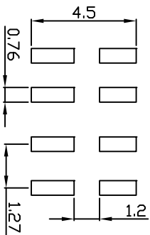
P. C. B Hole Layout
