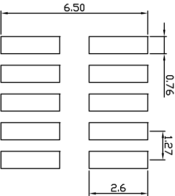
P. C. B. Hold Layout
