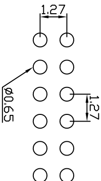
P. C. B Hole Layout
