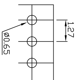
P. C. B Hole Layout
