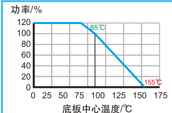
降功率曲线（热阻） Power reduction curve (thermal resistance): 5.71KW/K(0.18K/W)
